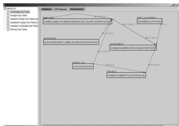
Figure 7: RID graph of the COMPANY database
