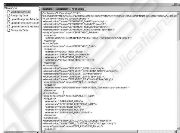
Figure 8: The output XML schema
