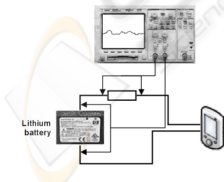
Figure 2: Circuit for measuring the energy consumed by the mobile device
