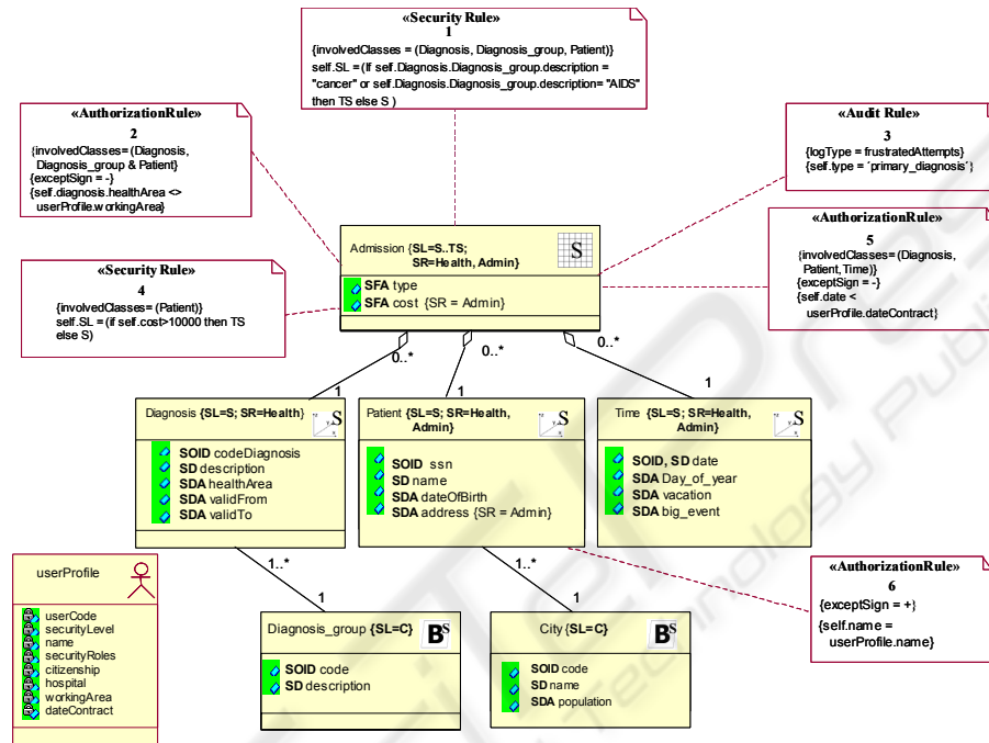
Fig. 5. Example of secure multidimensional modeling
