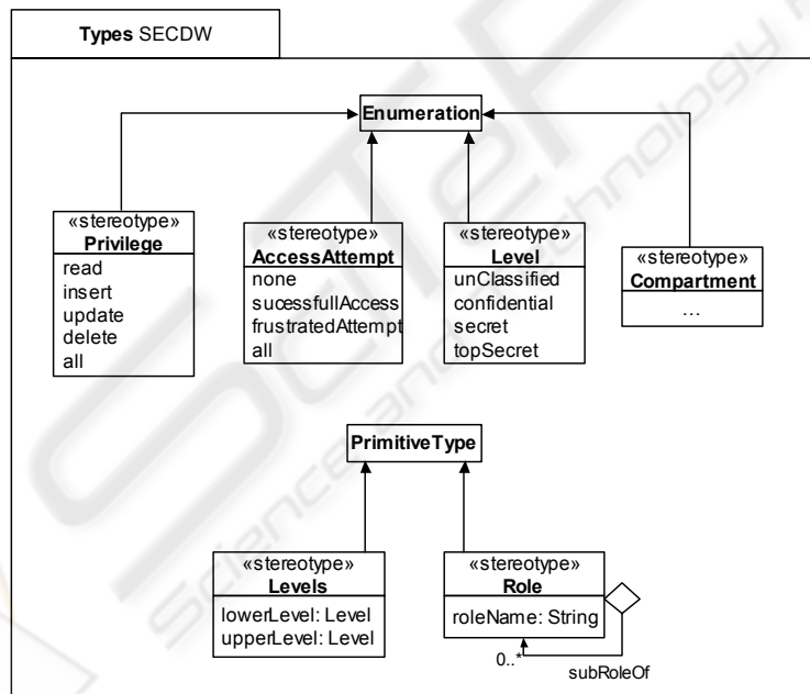
Fig. 2. Values associated to new data types
