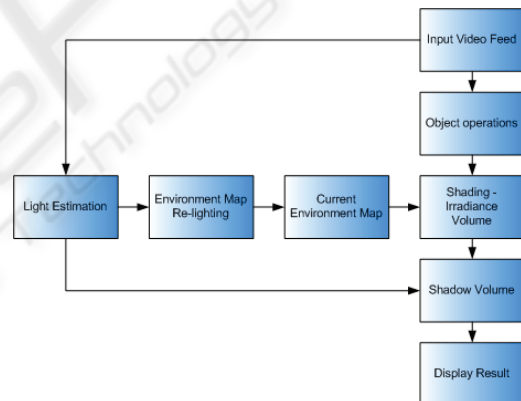
Figure 6: The online rendering pipeline used in the system.
