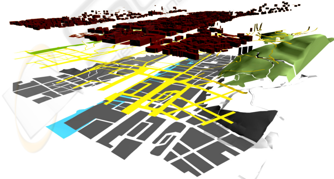
Figure 3: Terrain areas are separated into geometries representing the layers. To each layer geometry a different style can be applied. Buildings are placed on top of the terrain.
