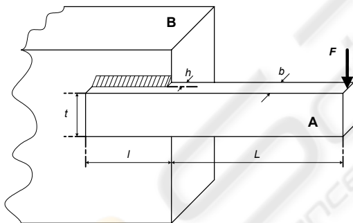
Figure 2: A Welded Beam.
