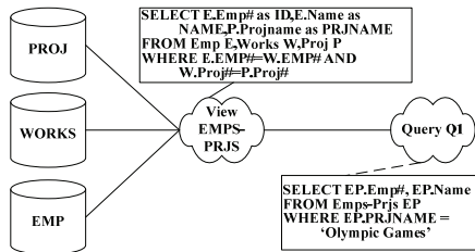
Figure 1: A simple configuration of a query over a view, defined over three relations.
