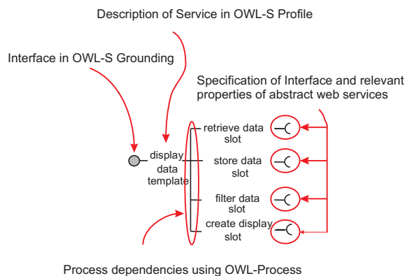
Figure 2: Template description in OWL-S.
