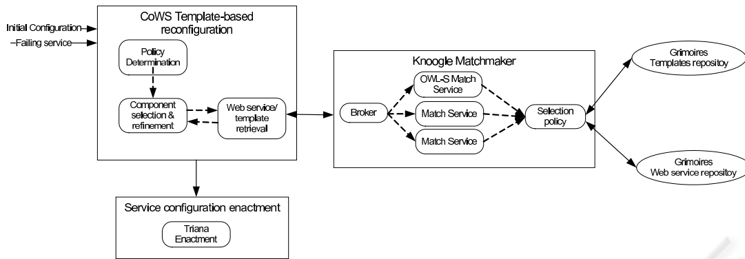
Figure 1: Architecture for dynamic service composition and enactment.
