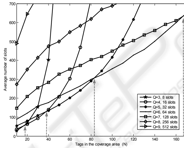
Fig. 1. Scenario 1. Identification rate vs number of tags for different values of Q .
