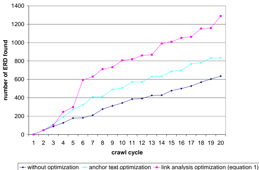
Figure 1: Crawl results with and without optimizations.
