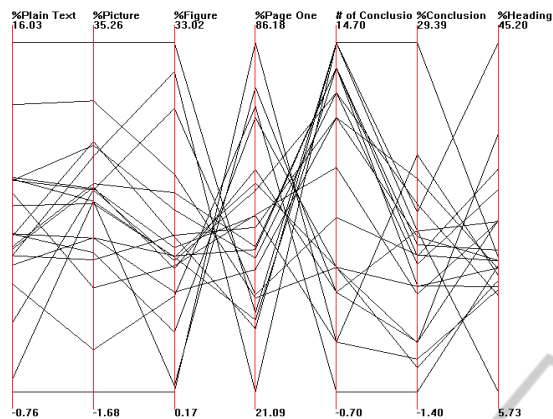
Figure 7: This image shows a parallel coordinates in XMDV (Ward, 1994). From left to right, the first four axes show the percentage of each participant's viewing time on plain text, pictures, figures and page one respectively. The last three axes show the number of conclusions each participant viewed, percentage of each participant's viewing time on conclusions and headings respectively.
