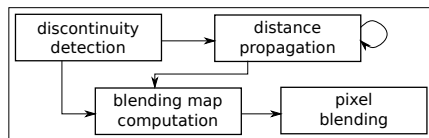
Figure 3: Algorithm overview.
