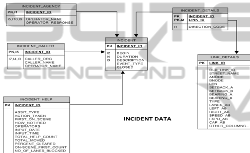
Figure 2: Star Schema for incident log.
