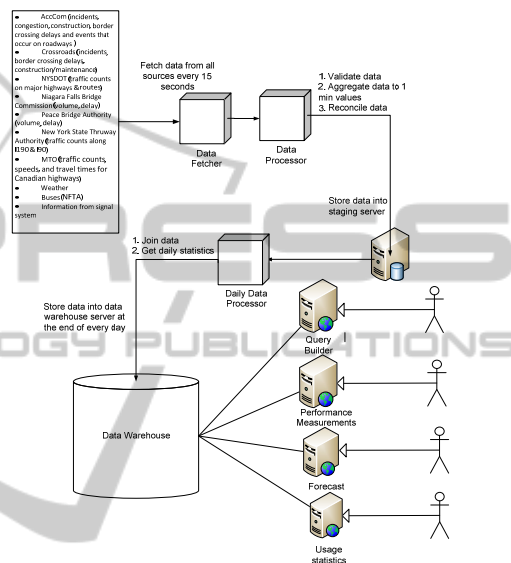
Figure 1: Data warehouse structure.
