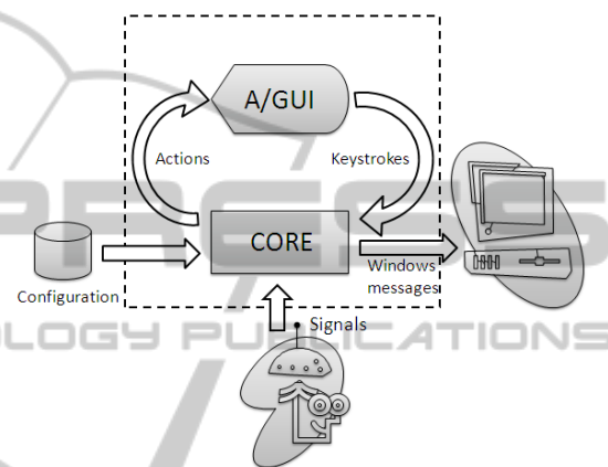
Figure 1: MindDesktop high level architecture.
