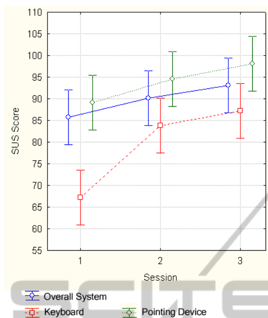
Figure 5: The SUS score reported by the users.
