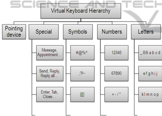
Figure 2: Input device state hierarchy.
