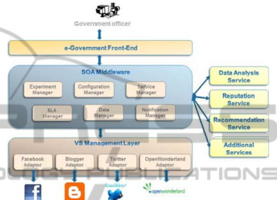
Figure 4: +Spaces architecture.
