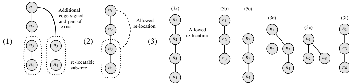
Figure 11: (1) Expanded tree with duplicates for all possible re-locations of sub-trees, (2) Tree with allowed Level-Promotion of n_3 , (3) Examples of valid trees with 3 or 4 nodes after: (3a) redact re-locatability, (3b) redact n_4 , (3c) redact root, (3d) relocate-only n_3 , (3e) re-locate n_3 and redact n_4 , (3f) redact n_2 and level-promote n_3 .
