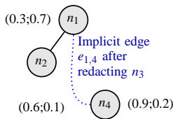
Figure 2: Intermediate Node Redaction T' following Kundu.
