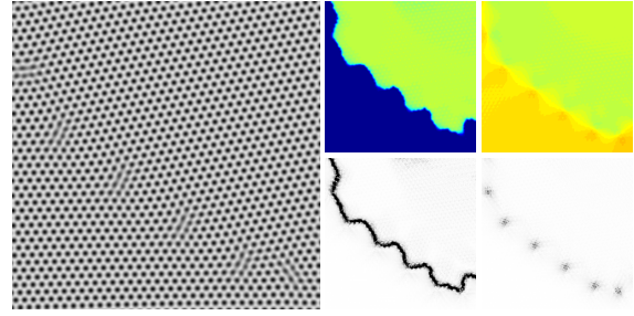
Figure 4: Original image and algorithm output for an initialization of F with rotations in [0, \pi/3] (left) and rotations in [\pi/6, \pi/2] (right). The top row shows the crystal orientation ( 0 \rightarrow \pi/2 , obtained via polar decomposition), the bottom row shows |\operatorname{curl} F| . The interpretation of the bottom left grain as being oriented at 0 rather than the equivalent \pi/3 leads to spurious curl.
