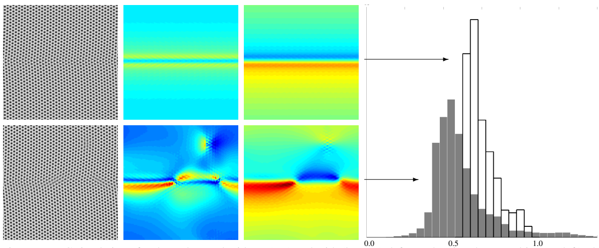
Figure 7: PFC simulation of a sheared crystal without (top) and with (bottom) defects, showing the crystal image (left), the elastic strain \text{dist}(F, \text{SO}(2)) (middle, 0 \leq \text{dist}(F, \text{SO}(2)) < 0.15 ), and F_{12} (right, -0.2 \leq F_{12} < 0.2 ). The rightmost graph shows a histogram of \text{dist}(F, \text{SO}(2)) . The crystal with defects has a higher peak strain, but lower overall strain.
