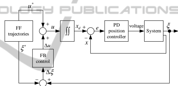
Figure 7: The 2-DOF control scheme for the swing-up.
