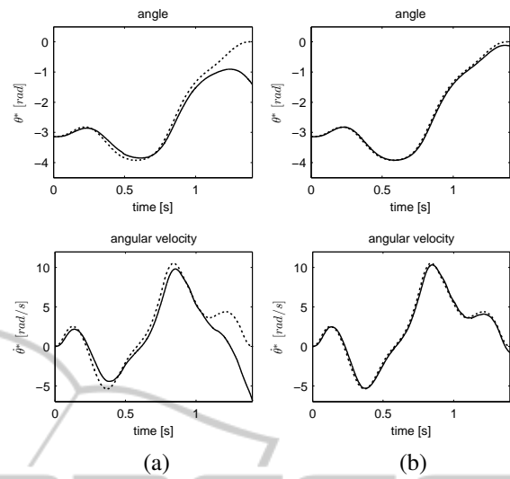
Figure 6: The open-loop experimental results for the angle and the angular velocity using (a) default parameters and (b) the estimated parameters.
