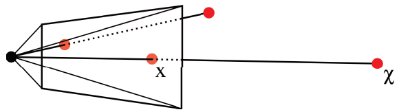
Figure 2: The projective camera model. A camera center and an image plane is defined. The image is formed by connecting a line between the camera center and the 3D point. The intersection between this line and the image plane defines the position of the projection for that 3D point.
