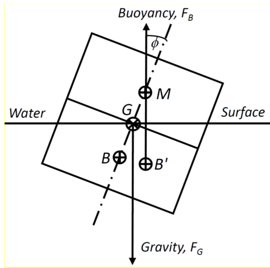
Figure 1: Stability principle.
