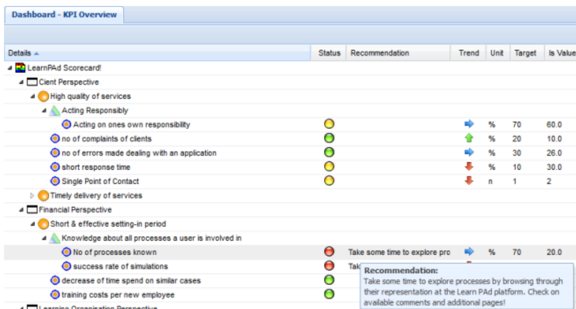
Figure 4: KPI dashboard with learning recommendation.
