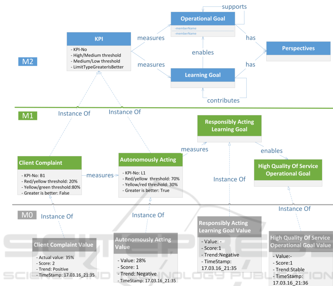
Figure 2: KPI model and instance layers.
