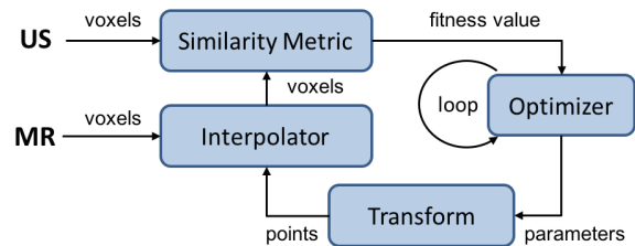
Figure 3: Diagram of the multi-modal registration module.
