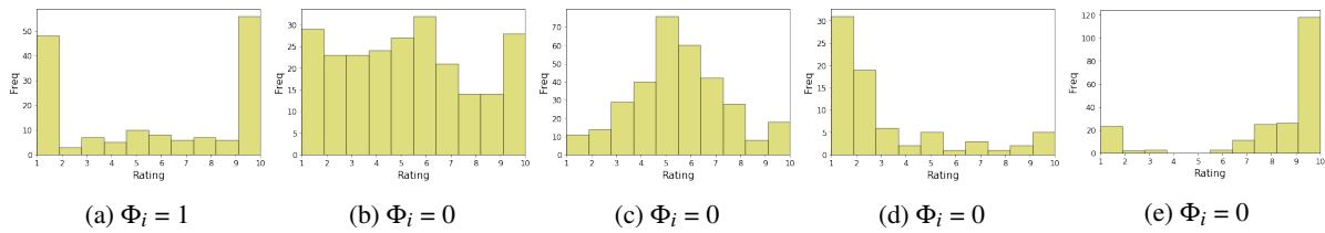
Figure 1: Polarization scores for different rating histograms.
