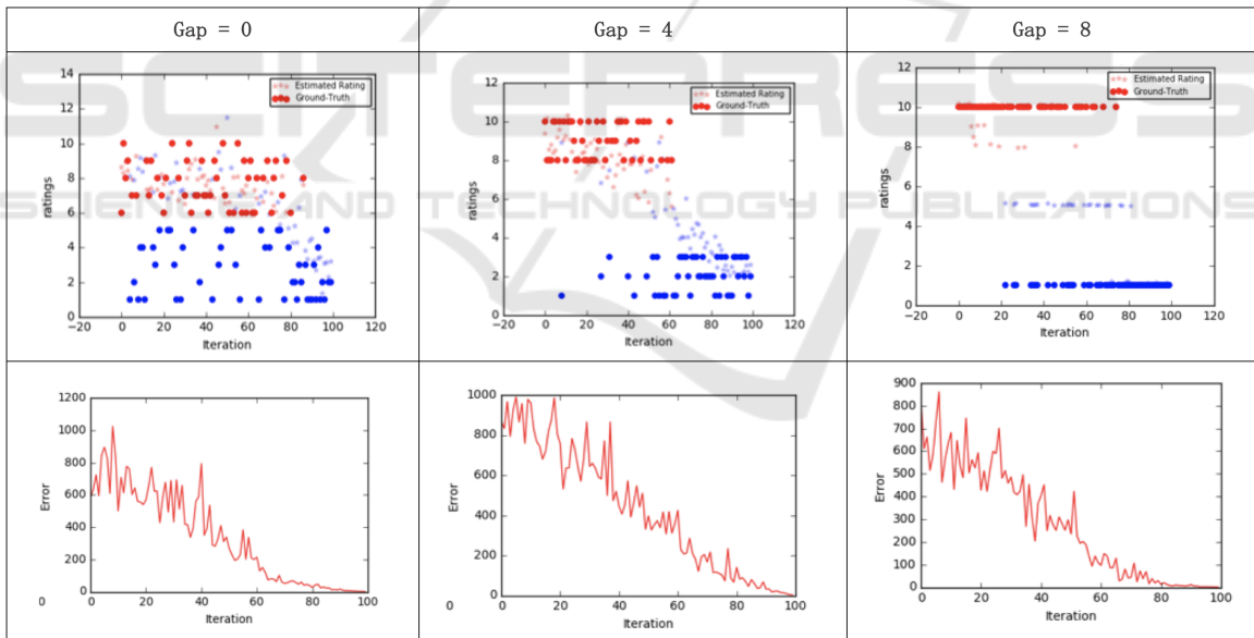
Figure 5: Traces of the Interactive Recommendation process when applying the pre-recommendation counter polarization (PrCP) strategy for user u_a . As we can see, the user gets to see items from different a color/view even in a very polarized environment.
