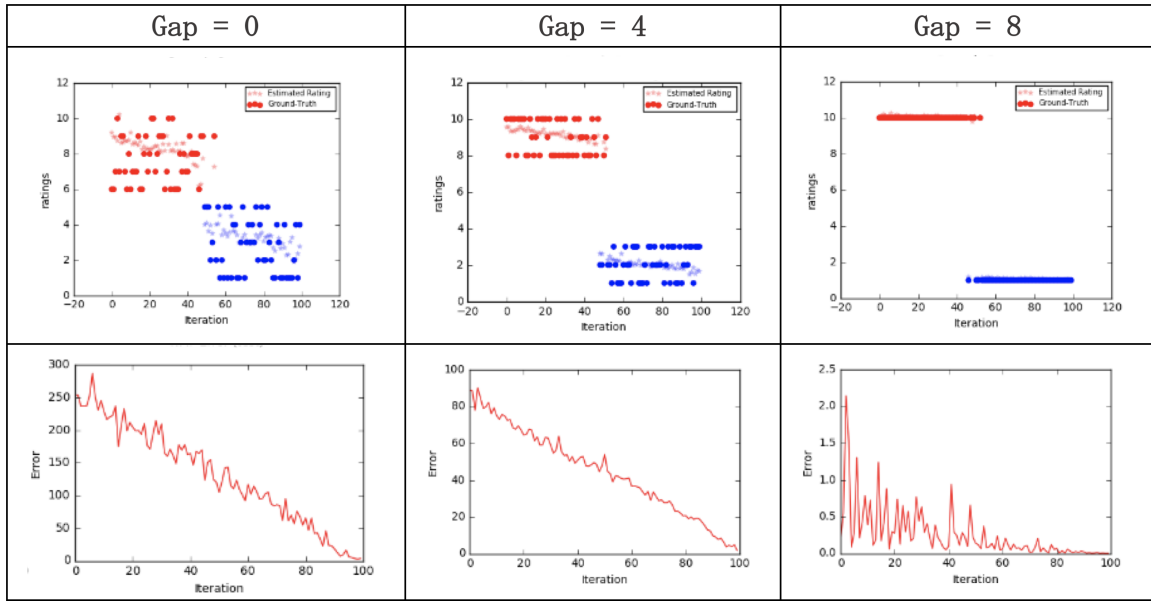
Figure 4: Traces of the Interactive Recommendation process with the classical NMF-based CF recommendation algorithm in environment G with different polarization ratio and gap values, for user u_a who had liked red items more. Although the red items are relevant, the user Red is trapped in a filter bubble that does not allow him/her to explore any items from the opposite color/view, at least not before the user has seen all of the Red items.
