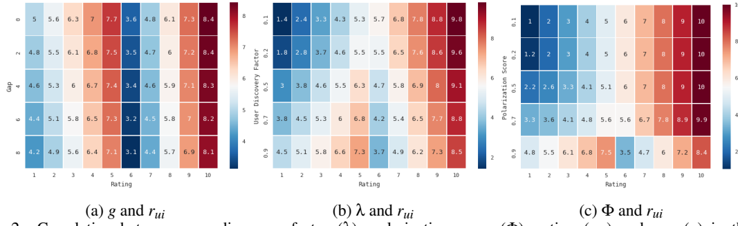
Figure 2: Correlation between user discovery factor ( \lambda ), polarization score ( \Phi ), rating ( r_{ui} ) and gap ( g ) in the pre-recommendation style counter-polarization approach.
