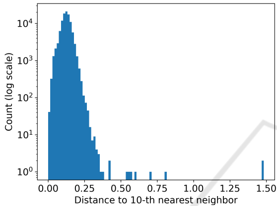
Figure 5: Histogram of the 10-th neighbour distances.
