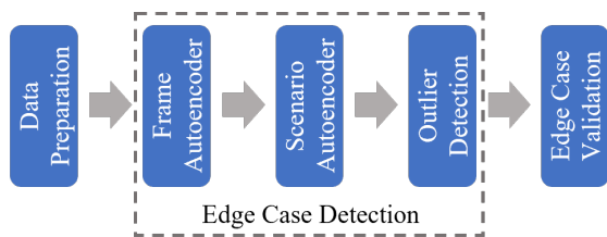
Figure 1: Edge Case Detection Method Overview.
