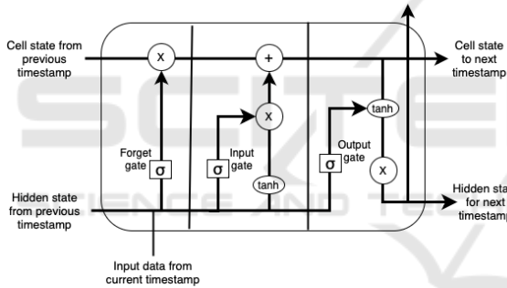
Figure 1: The structure of an LSTM memory cell.
