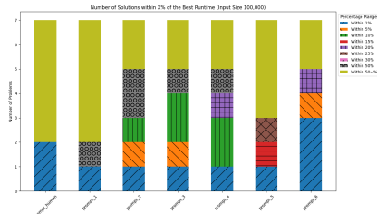
Figure 3: Number of Solutions within X% of the Best Runtime (Input Size 100,000).
