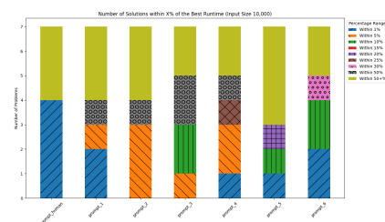
Figure 2: Number of Solutions within X% of the Best Runtime (Input Size 10,000).
