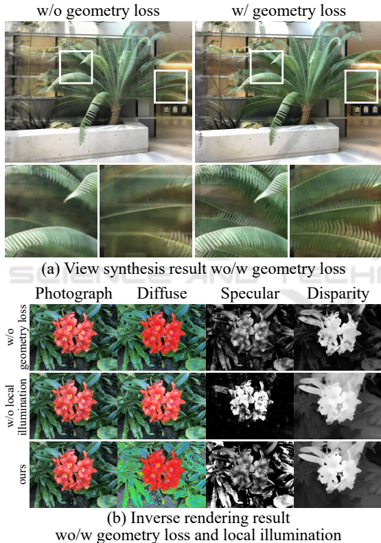
Figure 10: Ablation study. (a) Impact of the geometry loss in terms of image quality. (b) Impact of geometry loss and local illumination estimation for inverse rendering results.
