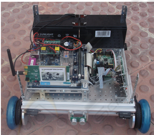
Figure 4a: Image of the robot
