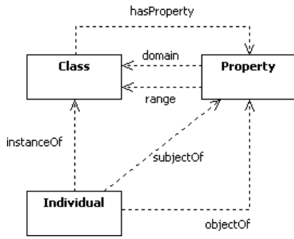
Figure 6: Logical components of the ontology model.
