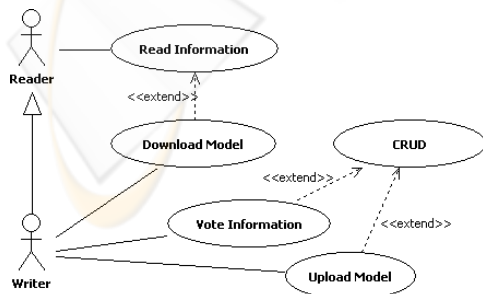
Figure 4: Web portal Writer use cases.
