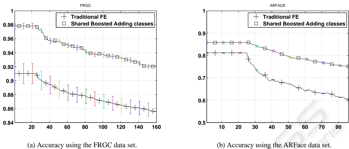
Figure 3: Accuracy as a function of the number of classes.
