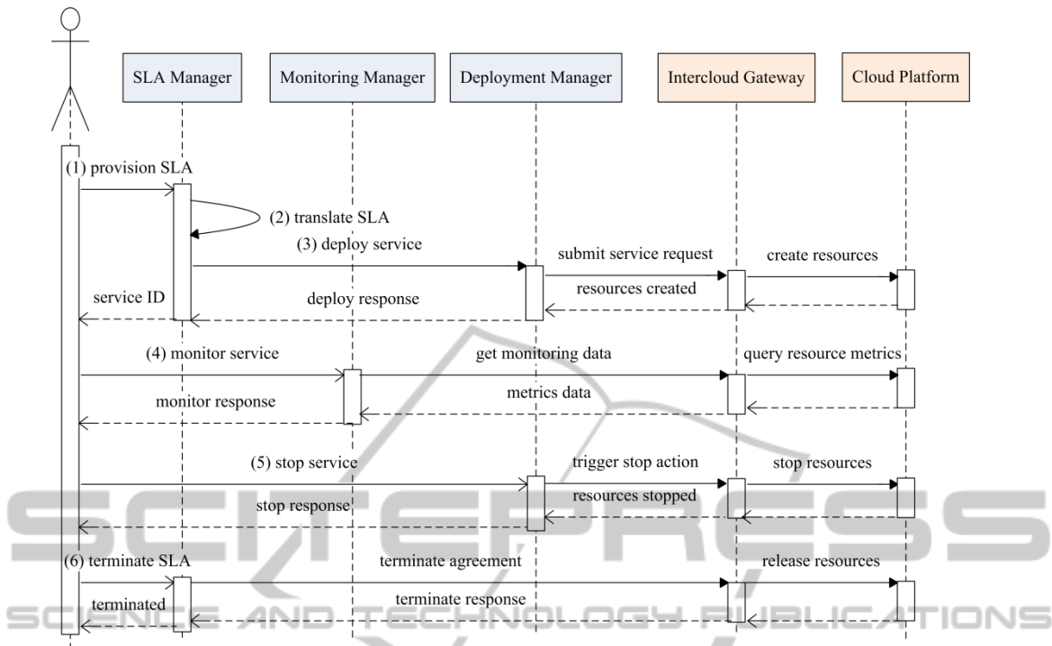
Figure 3: The SLA provisioning and monitoring flow.
