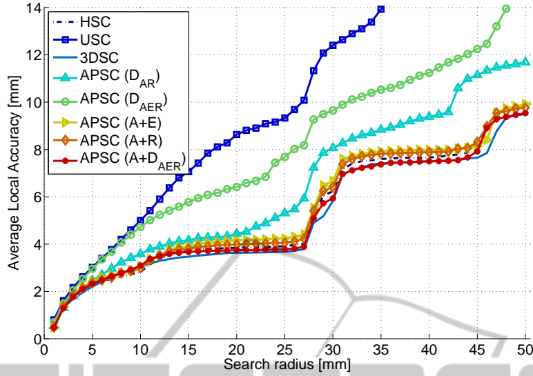
Figure 6: Average accuracy curves of all tested descriptors considering all landmarks together (by averaging).
