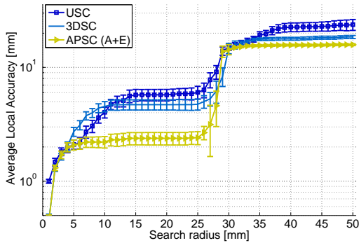
Figure 5: Average accuracy curves of USC, 3DSC and APSC (computing patterns over A + E rings) targeting the nose corners ( ac ). Error bars indicate a 95% confidence interval.
