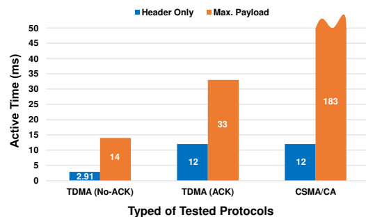
Figure 9: Comparison of minimum and maximum active time for three tested protocols in BRIX 2 module.
