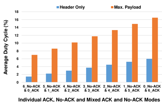
Figure 10: Comparison of the average duty cycle for ACK, No-ACK and mixed ACK and No-ACK modes.
