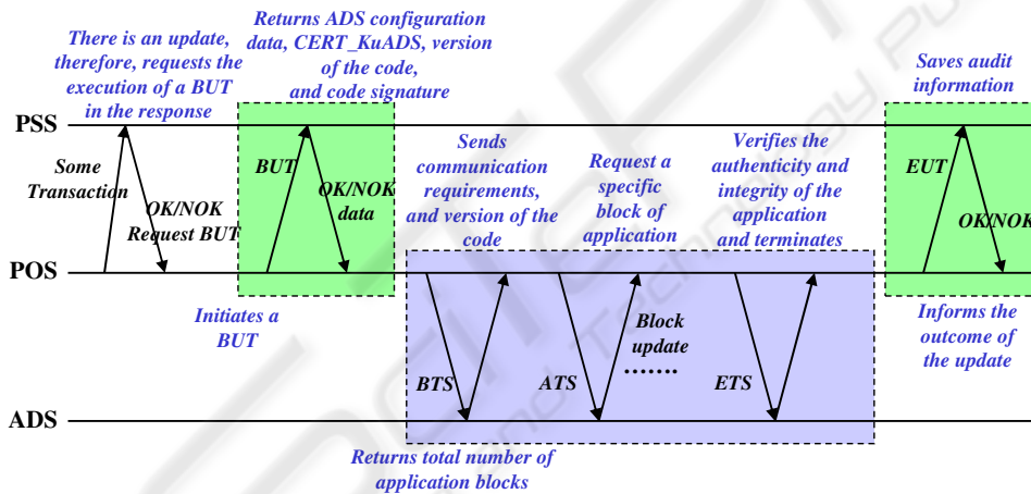
Figure 2: The update of an application.
