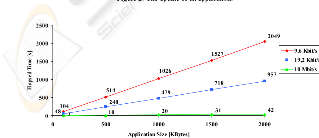
Figure 3: Elapsed time for the update of an application.
