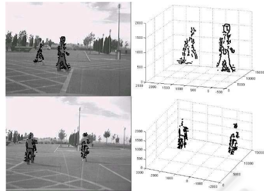
Figure 3: Left: 2D points into left image. Right: 3D points location.
