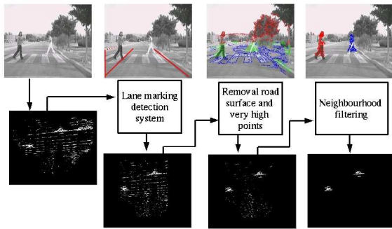
Figure 2: Filtering criteria and XZ maps.
