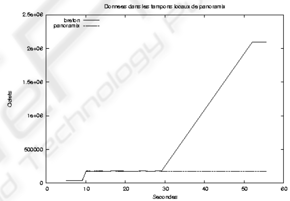
Figure 5: The buffers sizes of panoramix and breton when they run under Linux with a loaded system (from panoramix point of view)
