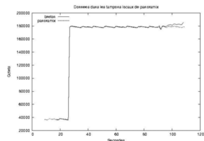
Figure 7 Buffers size of panoramix running under Bossa with a loaded system
