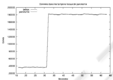
Figure 4: The behaviour of panoramix using Bossa and breton using Linux when the system is not loaded (from panoramix point of view)
