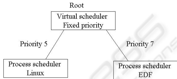
Figure 3: A scheduler hierarchy
