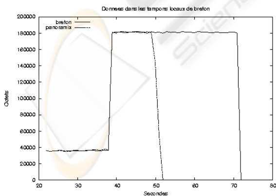
Figure 6: Buffers size of panoramix and breton running under Linux with a loaded system (from breton point of view)
