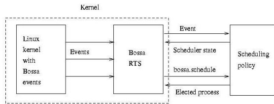
Figure 2: Bossa architecture
