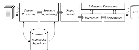
Figure 1: The production architecture.
