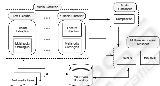
Figure 2: Classifying and storing multimedia items.
