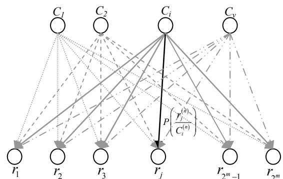
Figure 1: The proposed BN.
