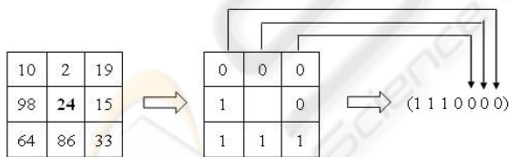
Figure 8: Example to calculate the binary label in LBP.
