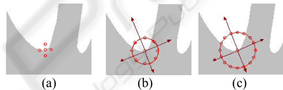
Figure 3: The proposed competitive hand valley detection algorithm.
