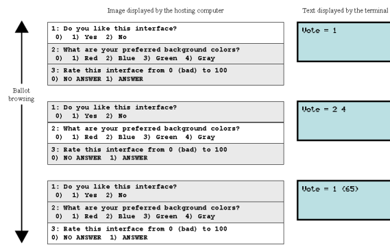
Figure 6: Ballot filling interface. On the left is the image presented by the hosting computer, which changes along the filling process and highlights the current question and all its possible answers. On the right is the text presented by the terminal — the answers to the current question.
