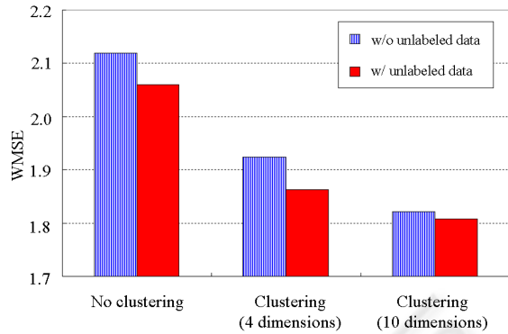
Figure 3: Comparison of WMSE (with/without clustering and supervised/semi-supervised learning).
