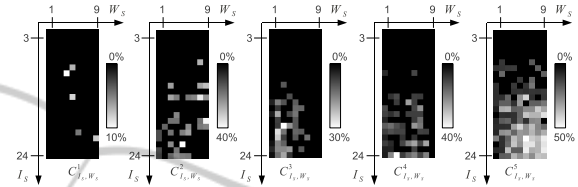
Figure 5: Each image shows how the F-measure varies in the parameter space (I_S, W_S) for each node C^1_{I_S, W_S} - C^5_{I_S, W_S} shown in Figure 3. A white pixel represents a F-measure equals to the maximum value. Each network was trained on 10 images of the training set and the F-measure was computed on the first 10 images of the testing set TU-Graz cars .
