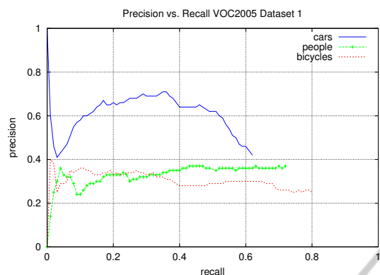
Figure 8: PR curve for the three classes of objects bicycles , people e cars . The model used for this graph is MNOD-SI.
