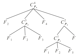
Figure 1: Generic structure of the proposed MNOD model. The nodes C_{\mathbf{P}}^n represent the supervised neural models which receive their input directly from the input features, the nodes F_i are the feature maps extracted from the input images.
