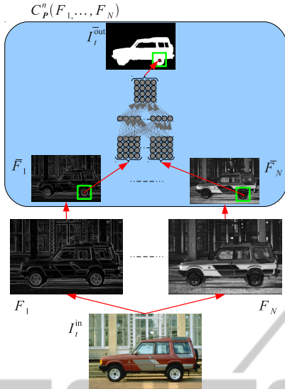
Figure 2: Generic structure of a node C_p^n(F_1, \dots, F_N) . The features F_1, \dots, F_N are created from each input images I_t^{in} . All the features images are re-sized in according to the parameter I_S \in \mathbf{P} in F_1, \dots, F_N . The output image I_t^{out} is hand-segmented and contains higher values for the pixels belonging to the objects of interest. The input patterns of the neural model are generated using a sliding window of size W_S \in \mathbf{P} which reads from the re sized images \bar{F}_1, \dots, \bar{F}_N , while the desired output is derived from the re sized output image \bar{I}_t^{out} .
