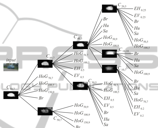
Figure 6: MNOD configuration used for the three categories of objects in the dataset VOC2005. The model displays the maps produced by each node C_p and the features used in input, all related to the input image of the testing set.
