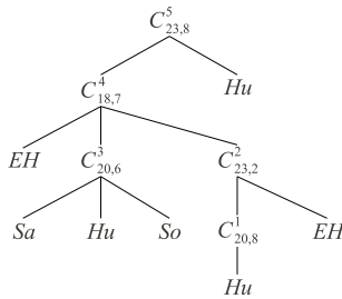
Figure 3: A configuration example where each node increases the accuracy measures (see Table 1 for details) using the output of child nodes.
