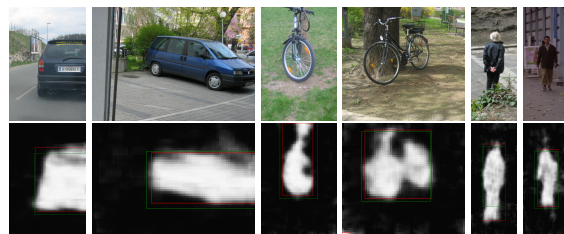
Figure 7: On the first line there are some image examples of the dataset VOC2005. On the second line the maps produced by the trained model and the desired bounding box in green.
