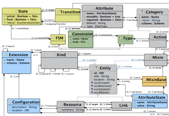
Figure 1: A subset of OCCIWARE METAMODEL.
