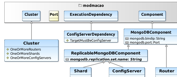
Figure 9: Modeling MongoDB with MoDMaCAO.
