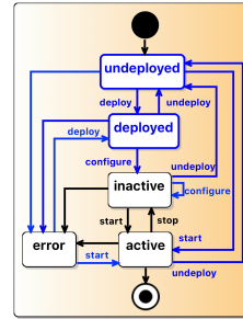
Figure 4: Enhanced OCCI Platform FSMs.
