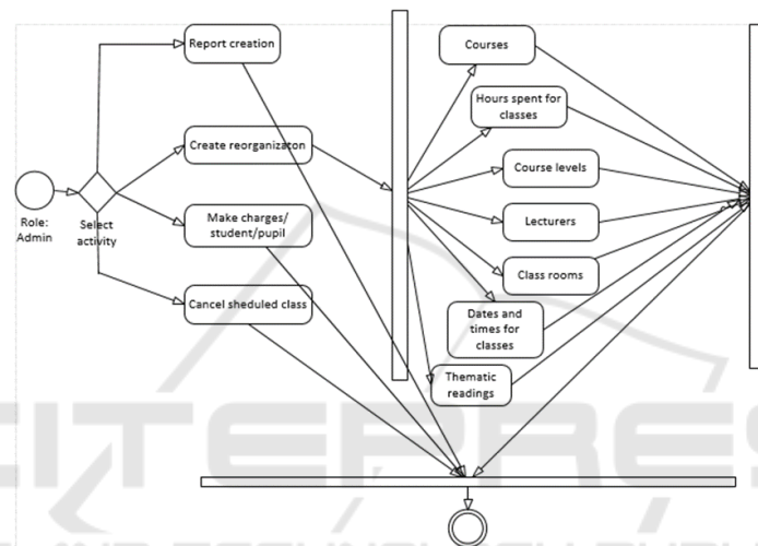
Figure 7: Proposed FMIS4CITE with activity diagram for the role Administrator.
